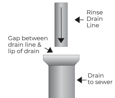
Figure 6 - Air Gap Illustration
