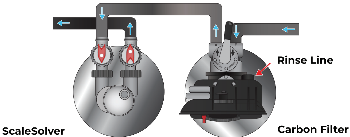
Figure 9 - Top view of the Premier PowerPac. Notice that the ScaleSolver inlet and outlet are reversed from water filter inlet and outlet.
