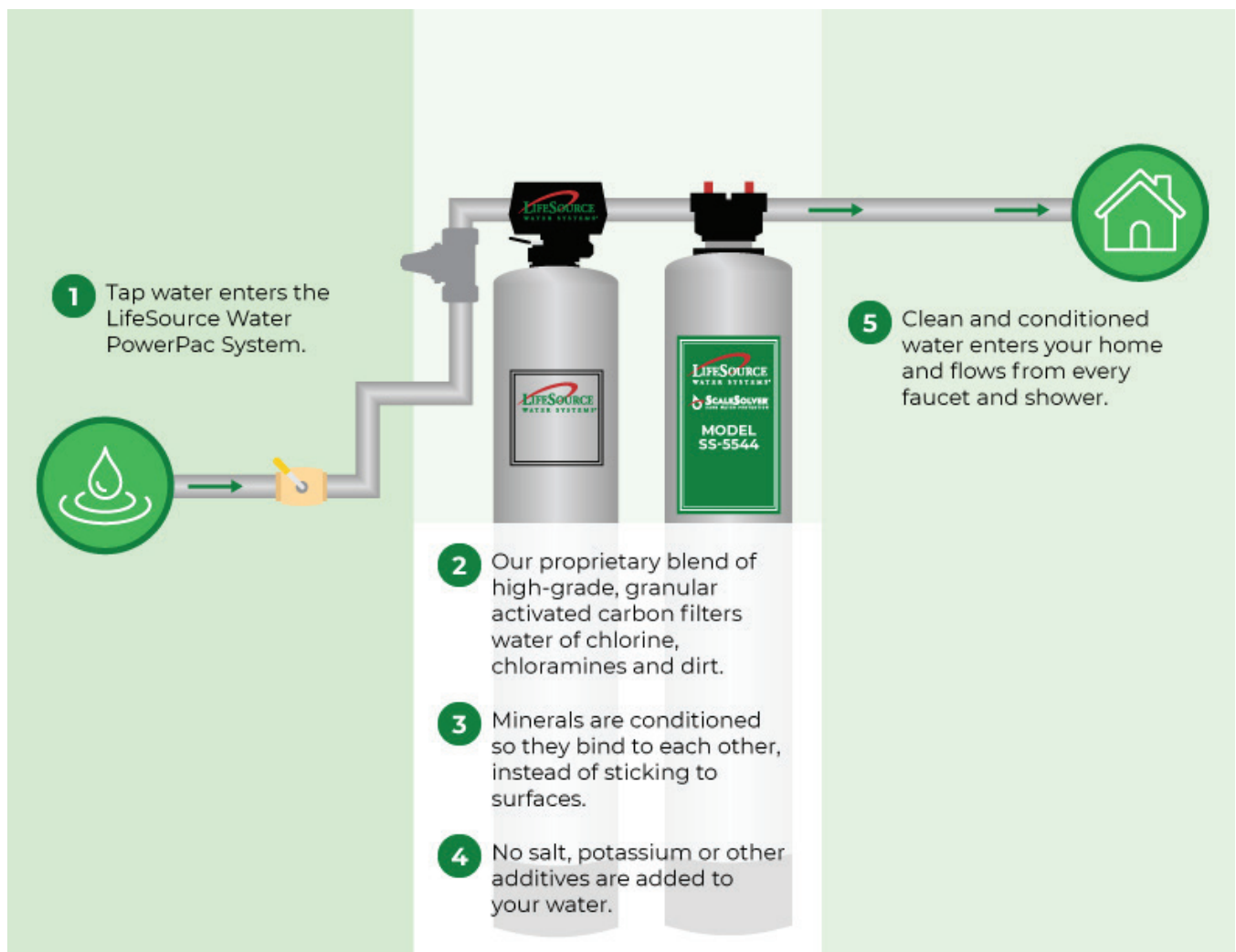
Figure 3 - PowerPac Water Loop Example
