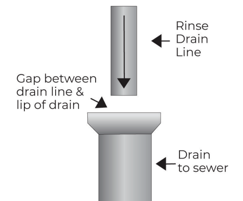
Figure 6 - Air Gap Illustration
