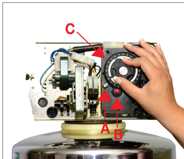
Figure 12 - Premier 2250SE timer
